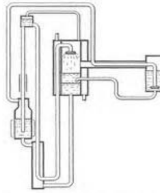
Einstein Refrigerator Patent number 1,672,812 - November 11, 1930 Alasdair MacLennan Ken Auld
